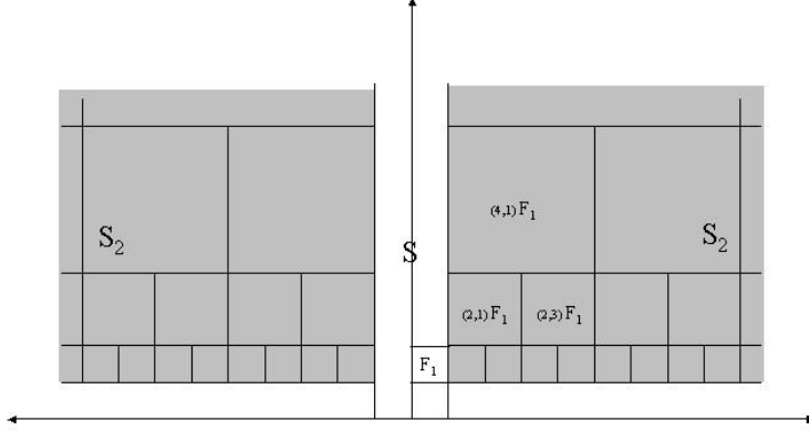
Figure 1: partition of S_2 into “equipotential” squares
